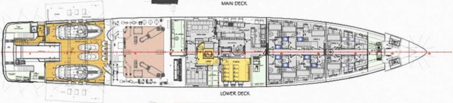
MAIN DECK
