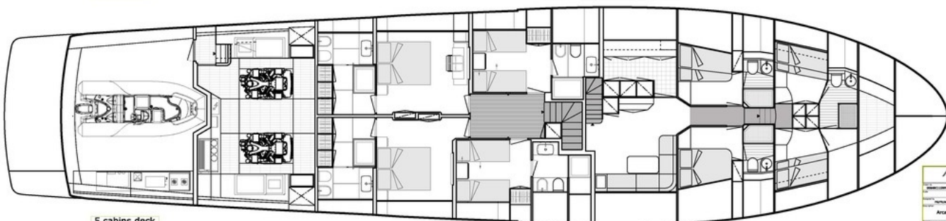
5 cabins deck
