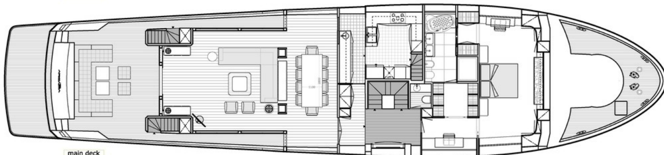
main deck
