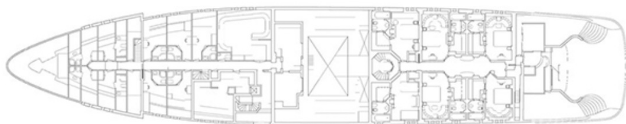
LOWER DECK
