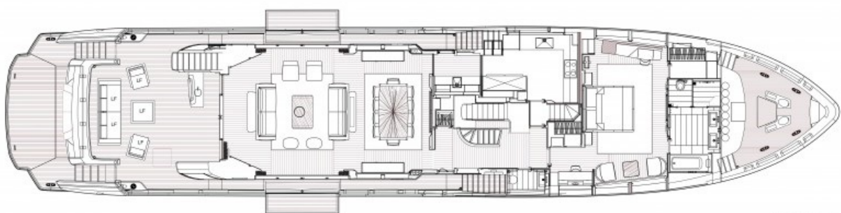
MAIN DECK PLAN (WITH OPTIONAL PORT/STARBORD BALCONY)
