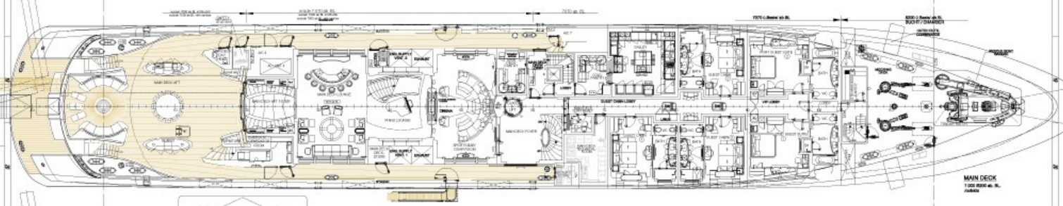
UPPER DECK 18,000 sq. ft. in area with corridor 12,000 sq. ft. in area
