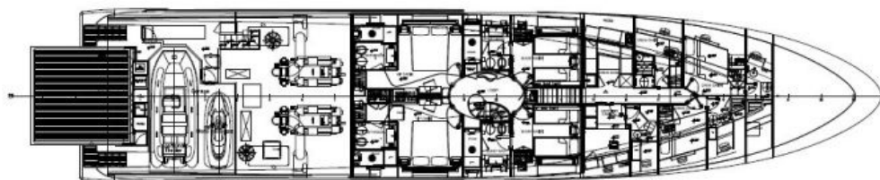
Lower deck
