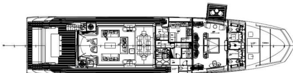
Main deck
