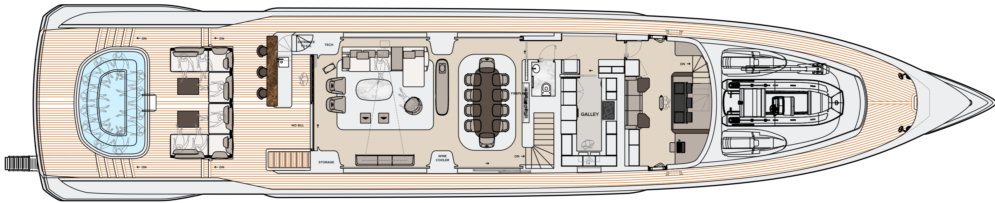
MAIN DECK
