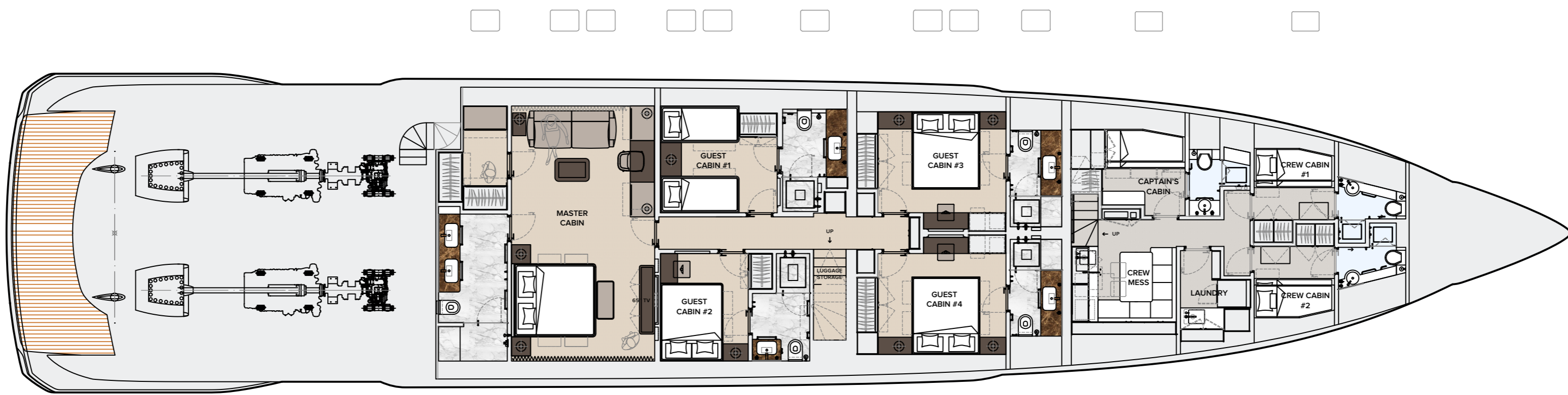
LOWER DECK
