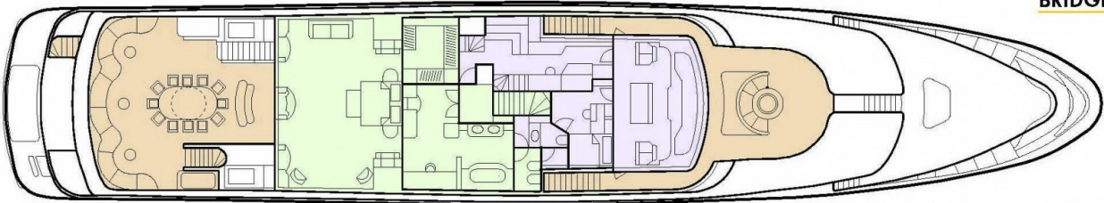
BRIDGE DECK
