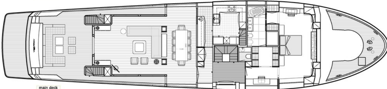
main deck
