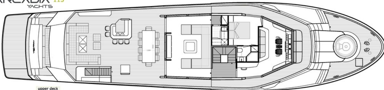
upper deck
