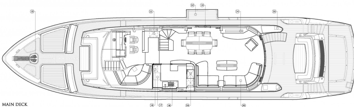
MAIN DECK
