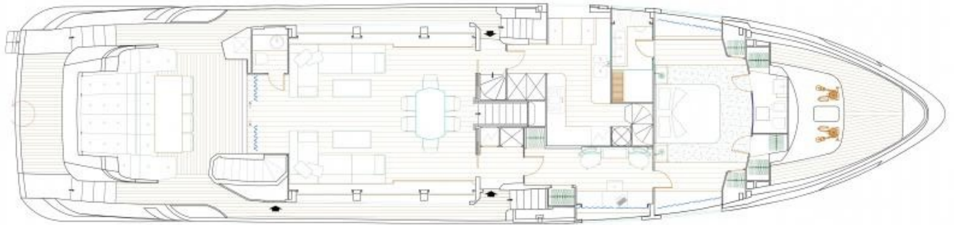
Main Deck
