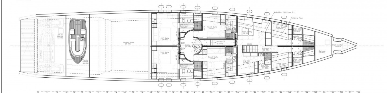
01 Lower Deck General Arrangement
