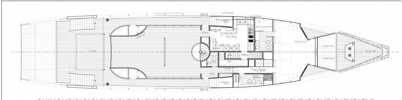
02 Main Deck General Arrangement
