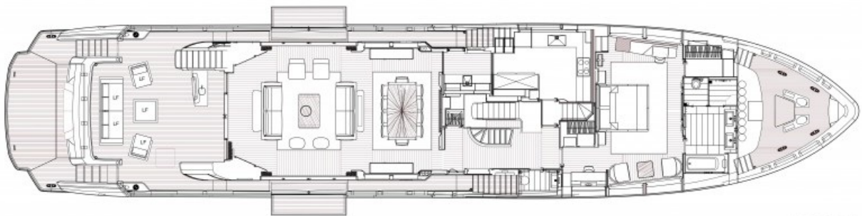
MAIN DECK PLAN (WITH OPTIONAL PORT/STARBORD BALCONY)
