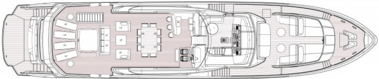
FLYBRIDGE PLAN
