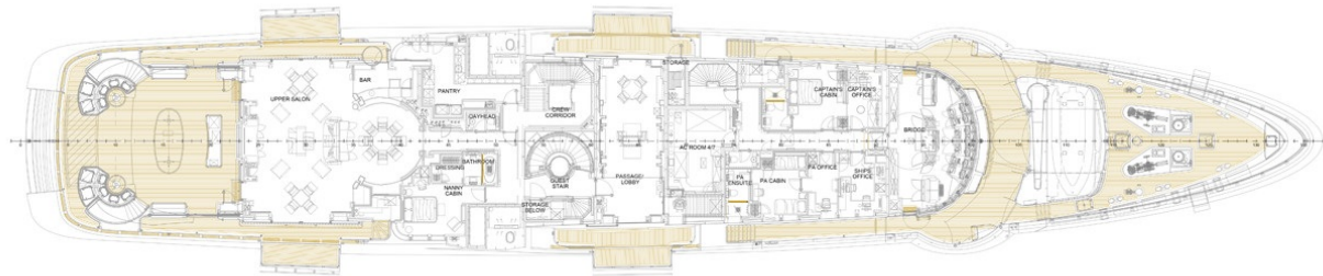
Wheelhouse Deck 040
