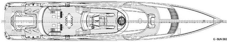
E - SUN DECK
