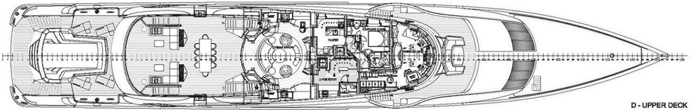
D - UPPER DECK
