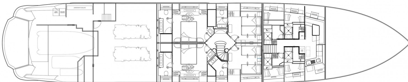
LOWER DECK
