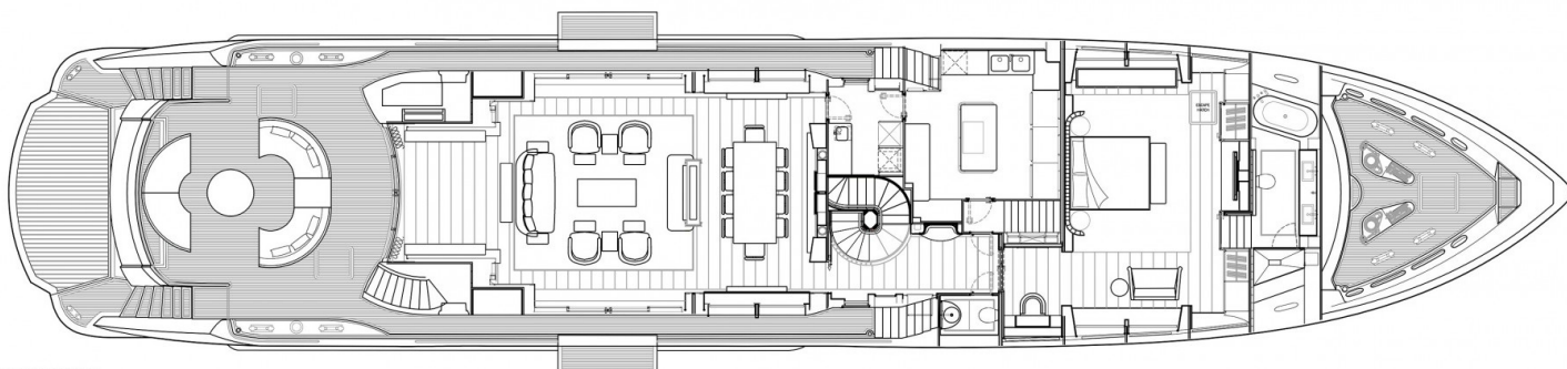
MAIN DECK
